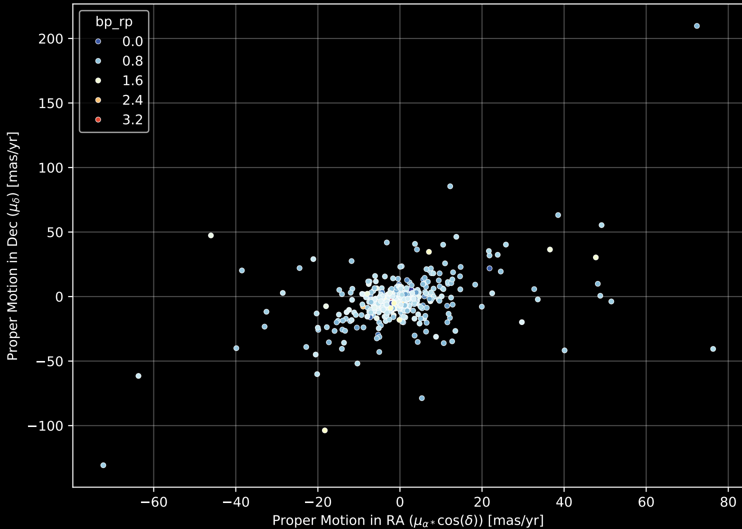
APOGEE DR17 Field: [K11_076+13] Proper Motion Diagram (n= 564)
