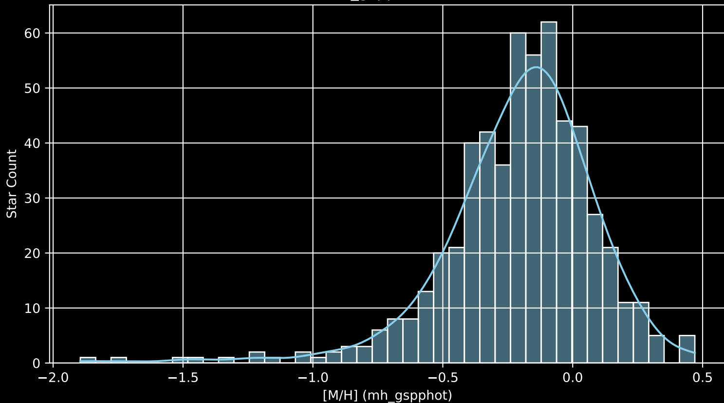
APOGEE DR17 Field: [K11_076+13 [M/H] (mh_gspphot) (n= 558)
