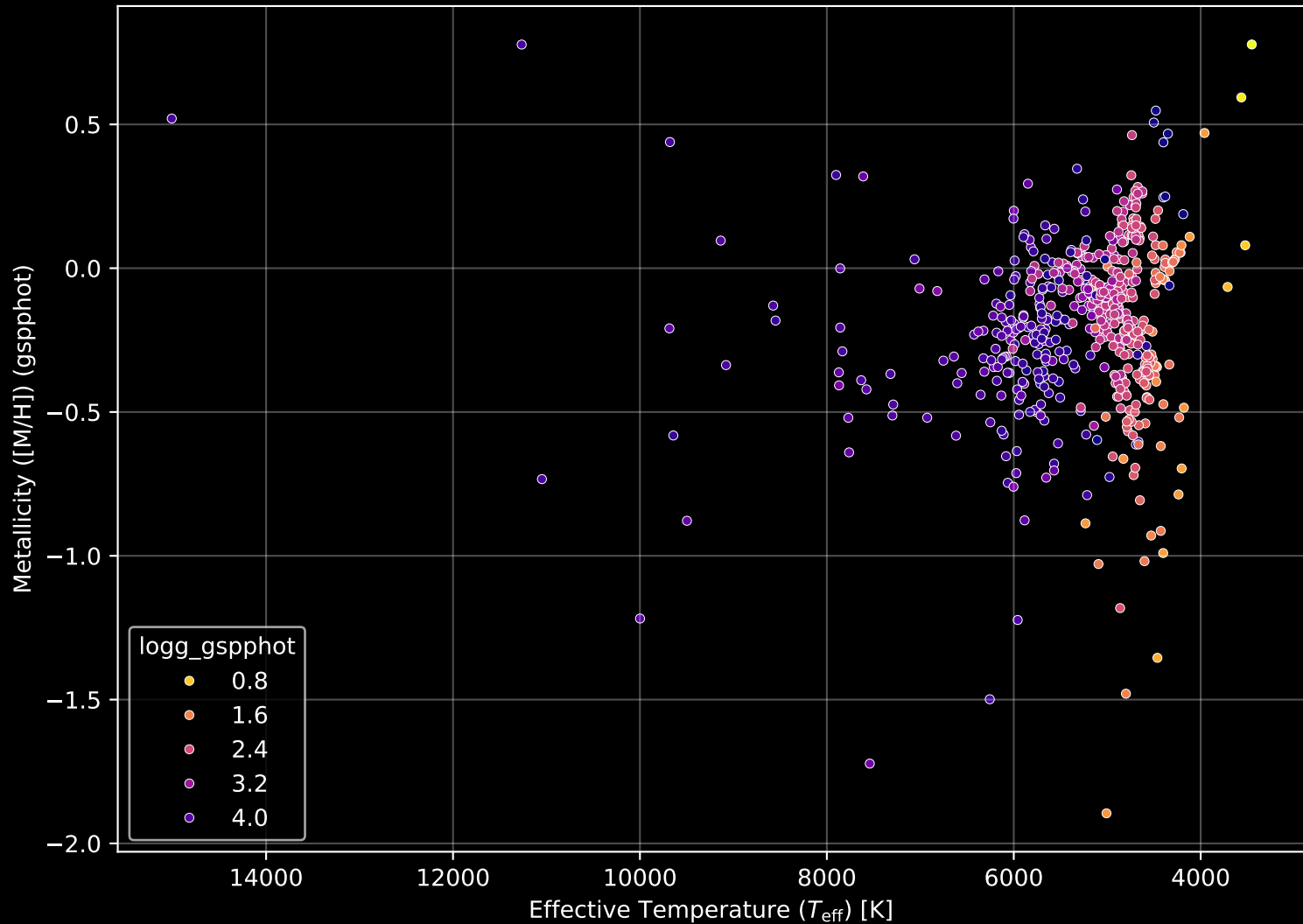
APOGEE DR17 Field: [K11_076+13] Stellar Population Parameters (n= 564)
