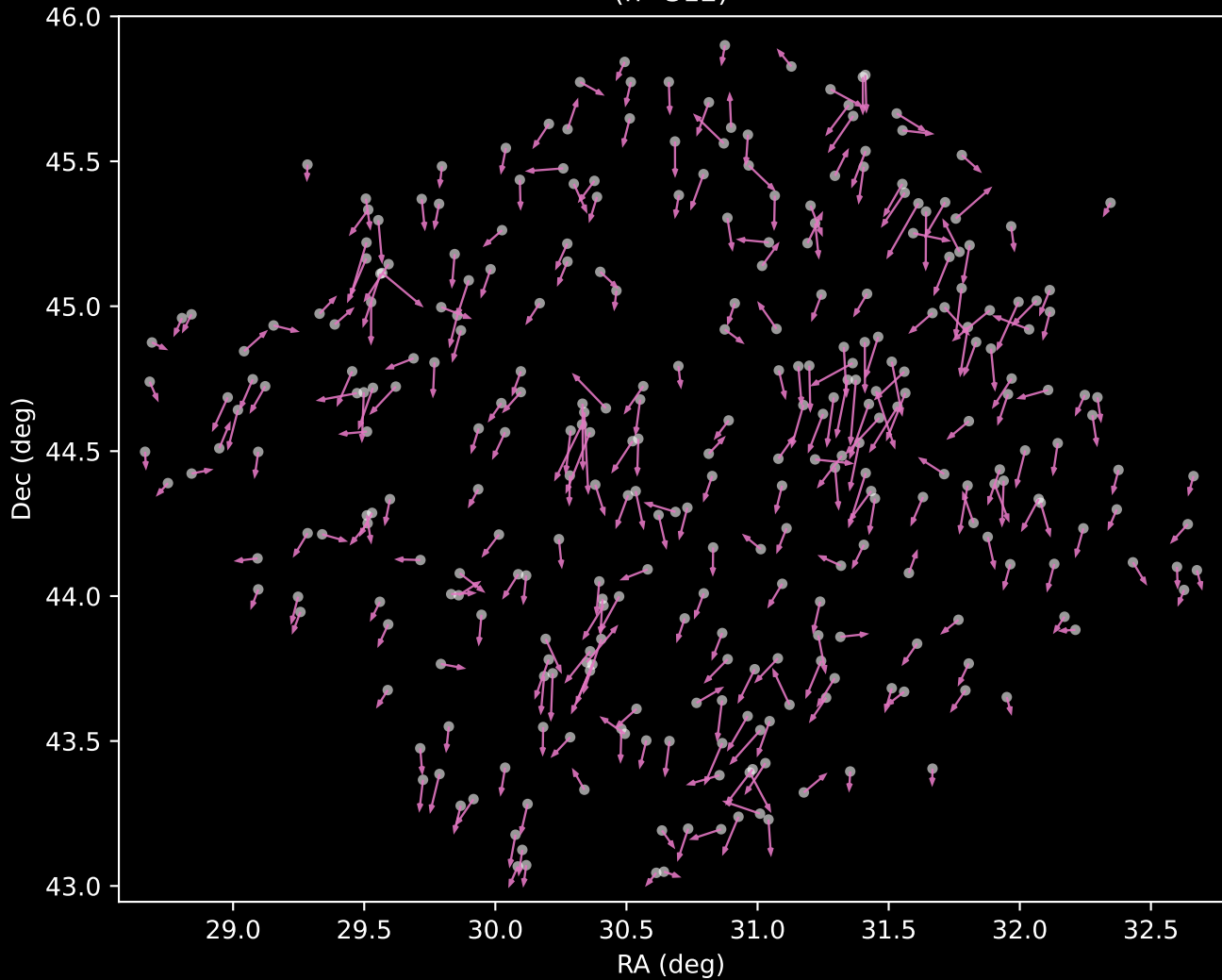
APOGEE DR17 Cluster 12 Proper Motion Vectors (n=312)
