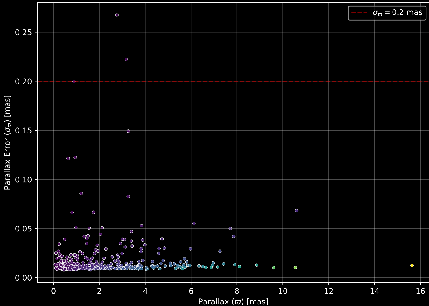
APOGEE DR17 Field: [K11_076+13] Parallax Quality (n= 564)
