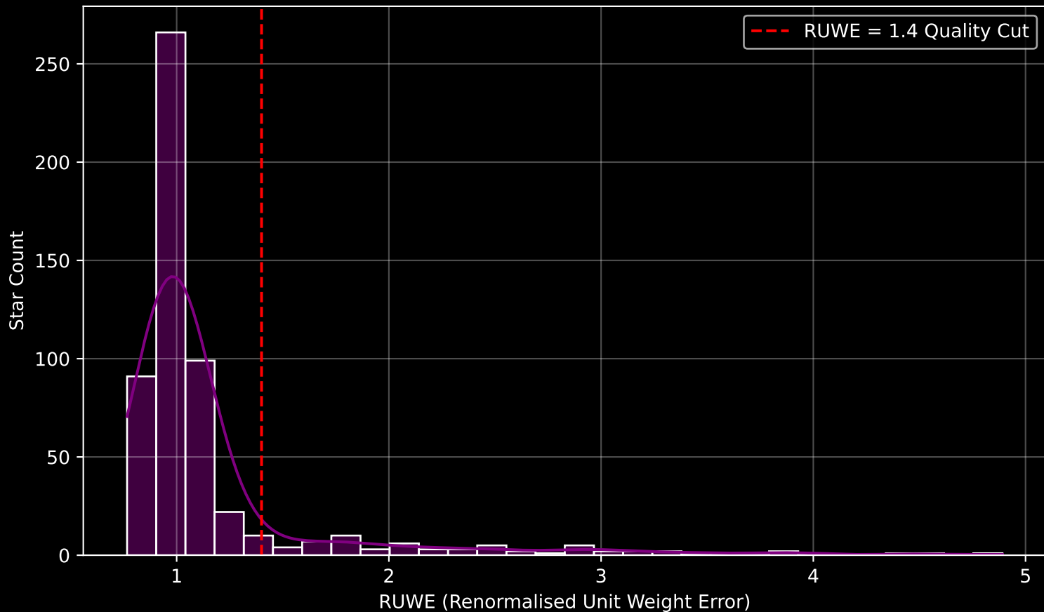
GAPOGEE DR17 Field [K11_076+13] RUWE Distribution (n= 552)
