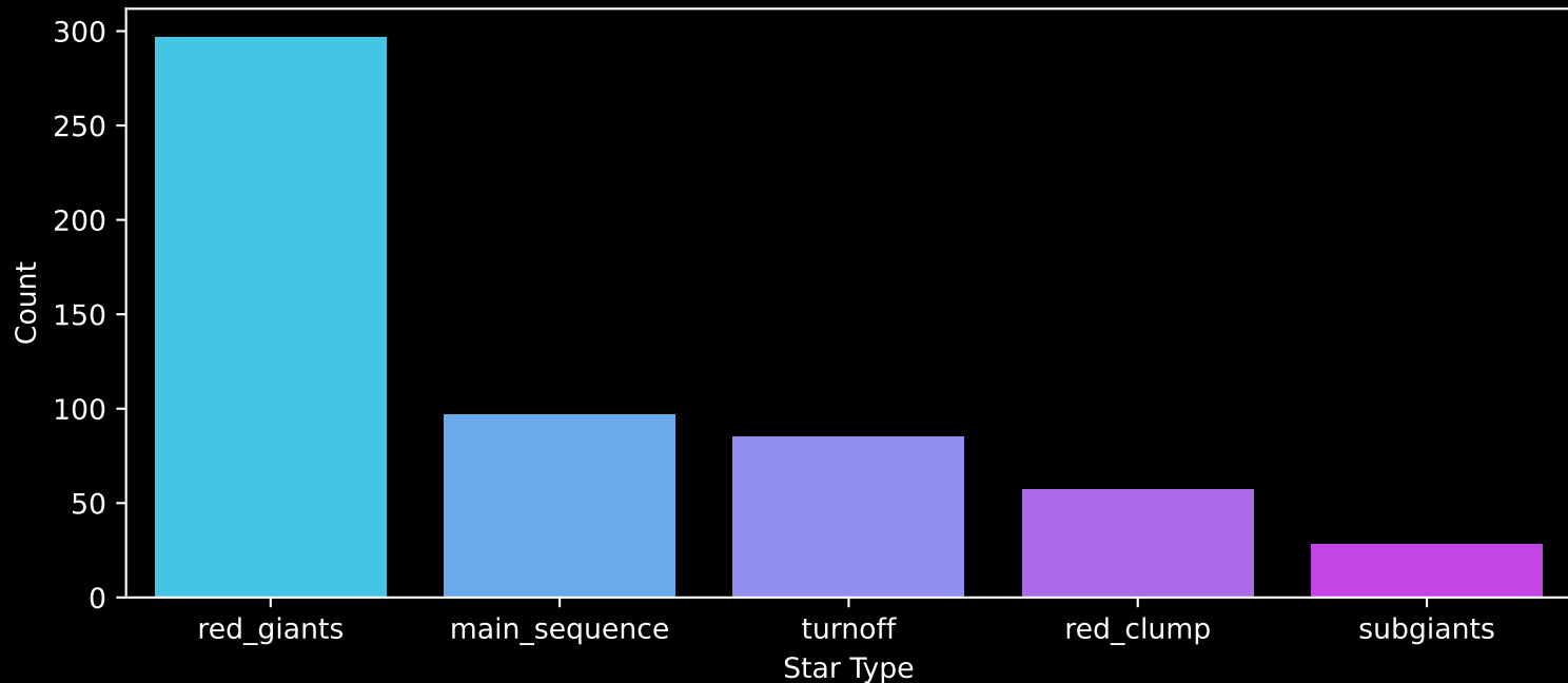
APOGEE DR17 Field: [K11_076+13] Count plot of Star Type
